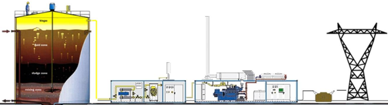
Digester / Reactor Gas Treatment Module Cogeneneration - Power Module Transformer Station
